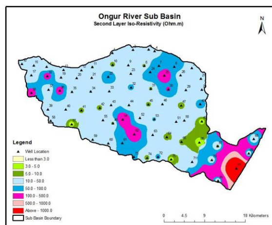
Fig.4. Second Layer Isoresistivity Map
